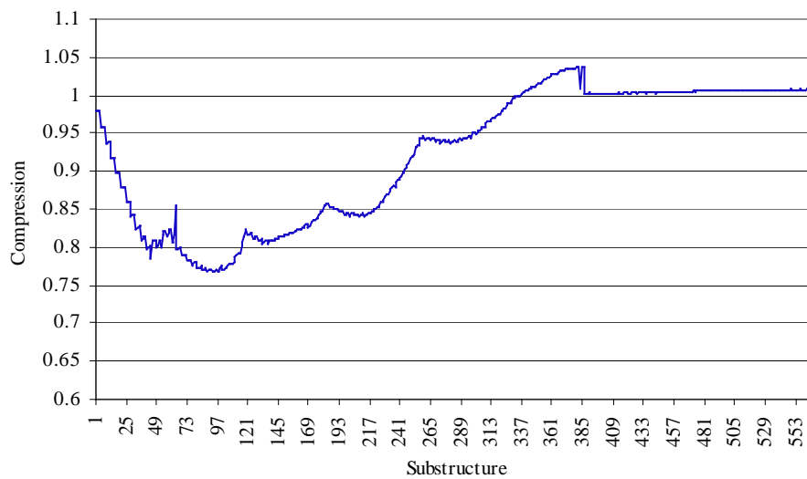
Figure 10: Compression of substructures as considered by SUBDUE during one iteration on an aircraft safety database.
