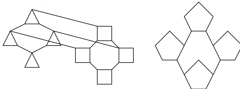
Figure 5: Artificial domain.
