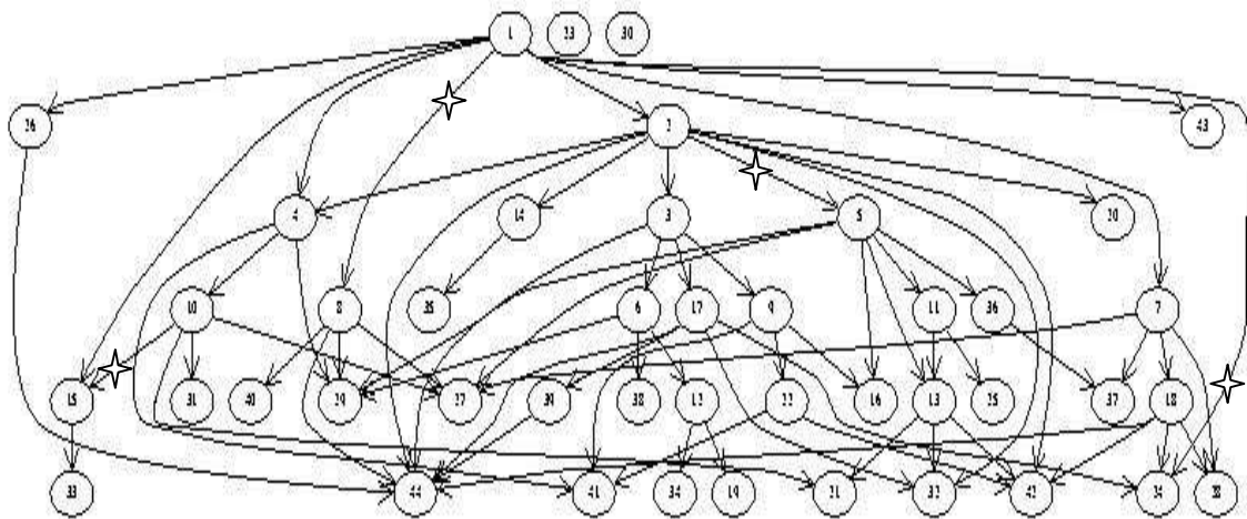
Figure 15. A portion of the web domain lattice generated by SUBDUE. Starred edges represent multiple edges between the pair of nodes.
